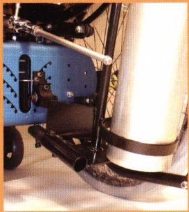
TheBUG OiS – Shown here with an Oxygen Cylinder adapter on the back of the frame. The cylinder articulates as the upper assembly is tilted.
